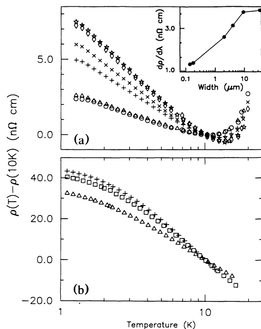
FIG. 1. The change in the low-temperature resistivity \rho(T) - \rho(10\text{ K}) for two sets of films of the same nominal impurity concentration. The depression of the Kondo resistance anomaly as the width is decreased is evident in both the 21.2- and 98.0-nm samples. The change in the residual resistivity from the widest to the narrowest films is only 9%. (a) A 21.2-nm 1000-ppm Cr in Cu film of width 0.14 ( \circ ), 0.16 ( \Delta ), 2.0 ( + ), 4.0 ( \times ), 9.5 ( \diamond ), and 35.0 \mu\text{m} ( \star ). Inset: d\rho/d\lambda for the six films plotted against the film width. (b) A 98.0-nm 1000-ppm Cr in Cu film of width 2.0 ( + ), 0.76 ( \square ), and 0.16 \mu\text{m} ( \Delta ). The depression of the Kondo anomaly with film thickness is evident from the difference in d\rho/d\lambda in the films of the same width and impurity concentration.
