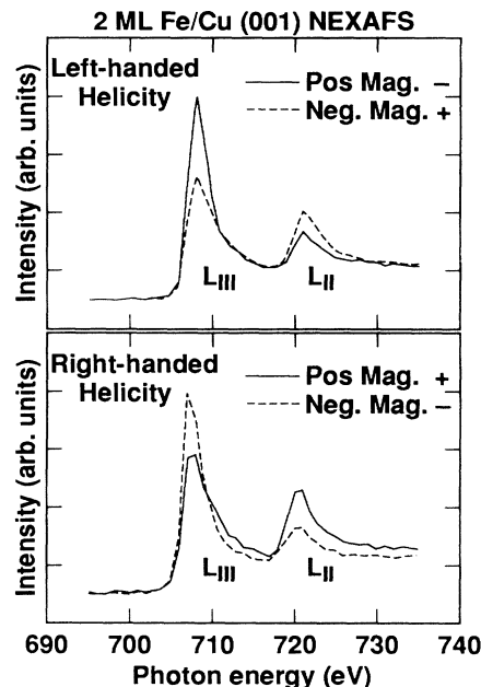
FIG. 1. The near-edge x-ray-absorption fine-structure (NEXAFS) dichroism of 2 ML of Fe/Cu(001). These are plots of absorption vs photon energy. The upper panel shows the effect of reversing the magnetization while maintaining the left-handed helicity of x rays. Similarly for the lower panel and right-handed helicity x rays. Samples are perpendicularly magnetized either into (positive magnetization) or out of (negative magnetization) the surface. The symbol + (-) means that the helicity and magnetization are parallel (antiparallel). The 2p^{3/2} peak is at the L_{III} edge and the 2p^{1/2} peak is at the L_{II} edge. The spectra were normalized to each other by equating the preedge intensity, at energies below approximately 700 eV.
