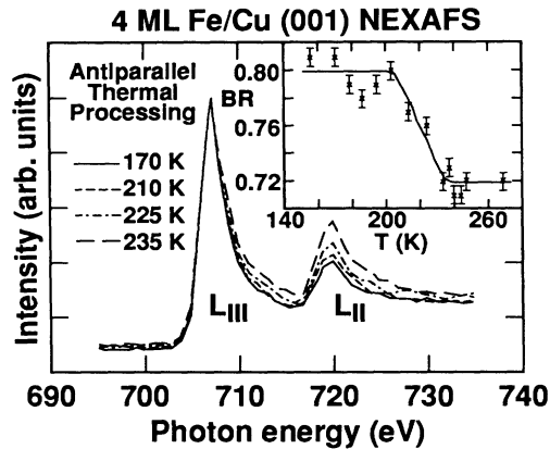
FIG. 2. The temperature dependence of the magnetization, using NEXAFS magnetic circular dichroism as the probe. Absorption vs energy spectra, similar to Fig. 1, are shown, as well as a plot of branching ratio (BR) vs temperature. The spectra are normalized to the maximum of the L_{III} peak. Because of imperfect placement of the thermocouple on the sample plate, the sample temperature may be slightly higher than that shown. Error bars of approximately \pm 1\% are included for comparison but the true error estimate is probably higher.
