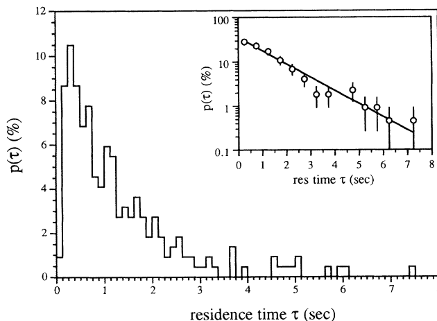
FIG. 2. Residence time probability distribution. Histogram of the distribution showing the exponential decay and the cutoff at short time. N = 219 events, \bar{\tau} = 1.3 sec, \sigma = 1.3 sec, skew = 2.0. Bin width \frac{1}{8} sec. Inset: Logarithmic plot showing weighted exponential fit to the data. \lambda_{fit} = 0.76 \pm 0.05 . Bin width = \frac{1}{2} sec.
