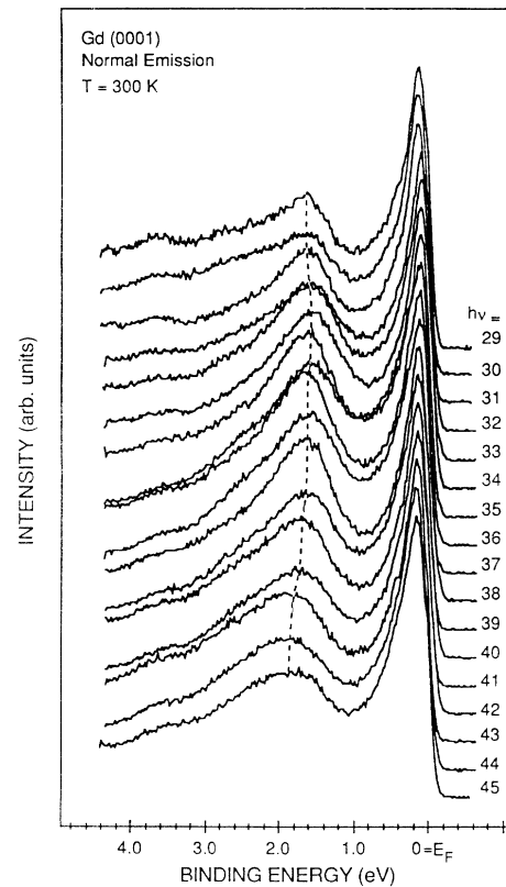
FIG. 2. Normal-emission photoelectron spectra from Gd(0001) for photon energies between 29 and 45 eV at 300 K ( T=1.02T_C ). The extremal peak position is assigned to the critical point \Gamma_4^- of the paramagnetic \Delta_2 band.
