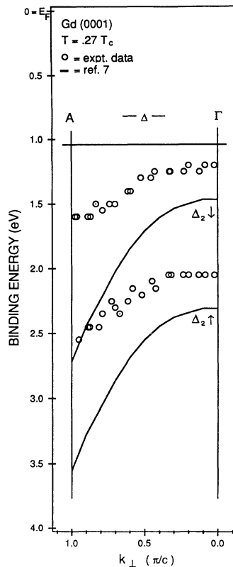
FIG. 3. Comparison of the calculated \Delta_2^{\uparrow} and \Delta_2^{\downarrow} energy bands of Ref. [7] with the experimental data of Fig. 1. The k_{\perp} position was determined using free-electron final-state bands. The lower branches of the \Delta_1^{\uparrow} and the \Delta_1^{\downarrow} bands from the \Gamma_1 + critical point are not shown.
