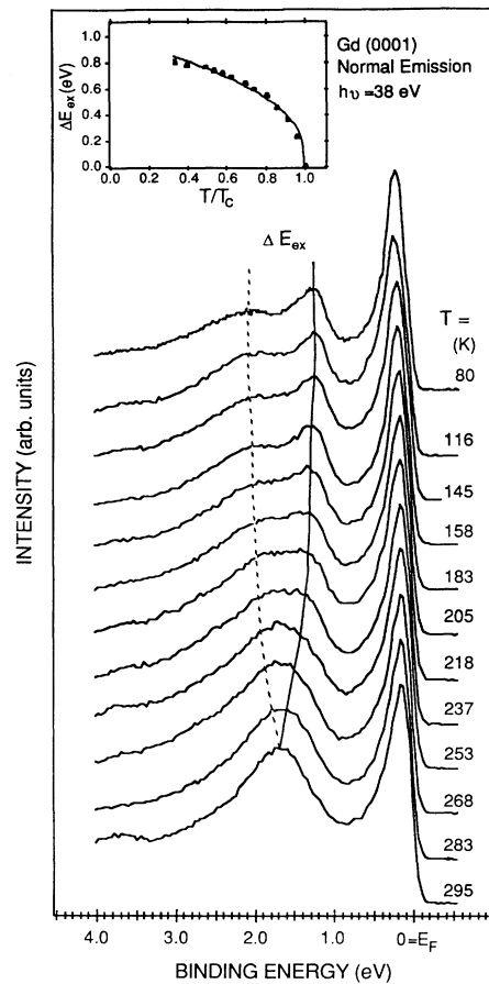
FIG. 4. Temperature dependence of the exchange splitting for the \Delta_2^{\uparrow} and \Delta_2^{\downarrow} energy bands between T = 0.27T_C and T = T_C at fixed k_{\perp} for the photon energy h\nu = 38 eV. Inset: Plot of peak positions vs reduced temperature, and curve fitted using a power law of the form \Delta E_{\text{ex}} = (1 - T/T_C)^{\beta} . The value obtained for the critical exponent \beta is 0.378, a value close to the exponent predicted by the Heisenberg model ( \beta \sim 0.35 ) and also close to the experimental result ( \beta \sim 0.40 ) for Gd obtained from magnetization measurements [16].
