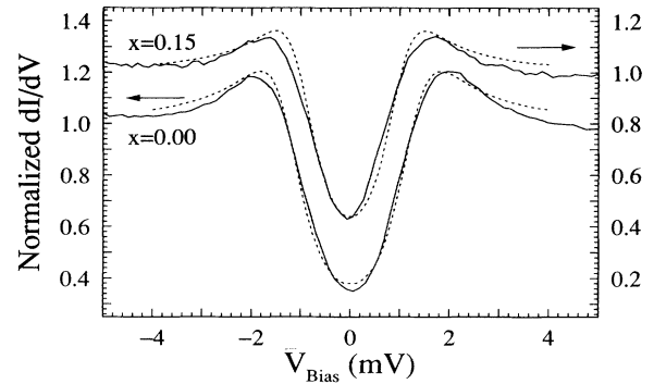
FIG. 2. Spectra acquired away from the flux lines at 1.3 K and 0.3 T for x=0.00 and x=0.15 . A fit by a pair-breaking model of the density of states is indicated by the dashed lines. The fitting parameters are, for x=0 , \Delta=1.3 \text{ meV} , \Gamma=0.51 \text{ meV} , and for x=0.15 , \Delta=1.0 \text{ meV} , \Gamma=0.46 \text{ meV} . In both cases the temperature is taken to be T=1.3 \text{ K} .
