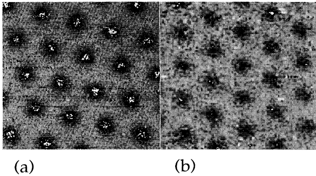
FIG. 1. 4000 \text{ \AA} \times 4000 \text{ \AA} STS images of the vortex lattice at 1.3 K and 0.3 T: (a) x=0.00 sample (pure \text{NbSe}_2 ); note that regions in which the conductance ratio is greater than 1 have been artificially saturated to white to highlight the spatial extent of the ZBCP in the vortex cores. (b) x=0.20 ; the ZBCP is absent in this case.
