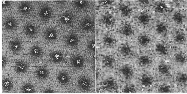
FIG. 1. 4000 \text{ \AA} \times 4000 \text{ \AA} STS images of the vortex lattice at 1.3 K and 0.3 T: (a) x=0.00 sample (pure \text{NbSe}_2 ); note that regions in which the conductance ratio is greater than 1 have been artificially saturated to white to highlight the spatial extent of the ZBCP in the vortex cores. (b) x=0.20 ; the ZBCP is absent in this case.
