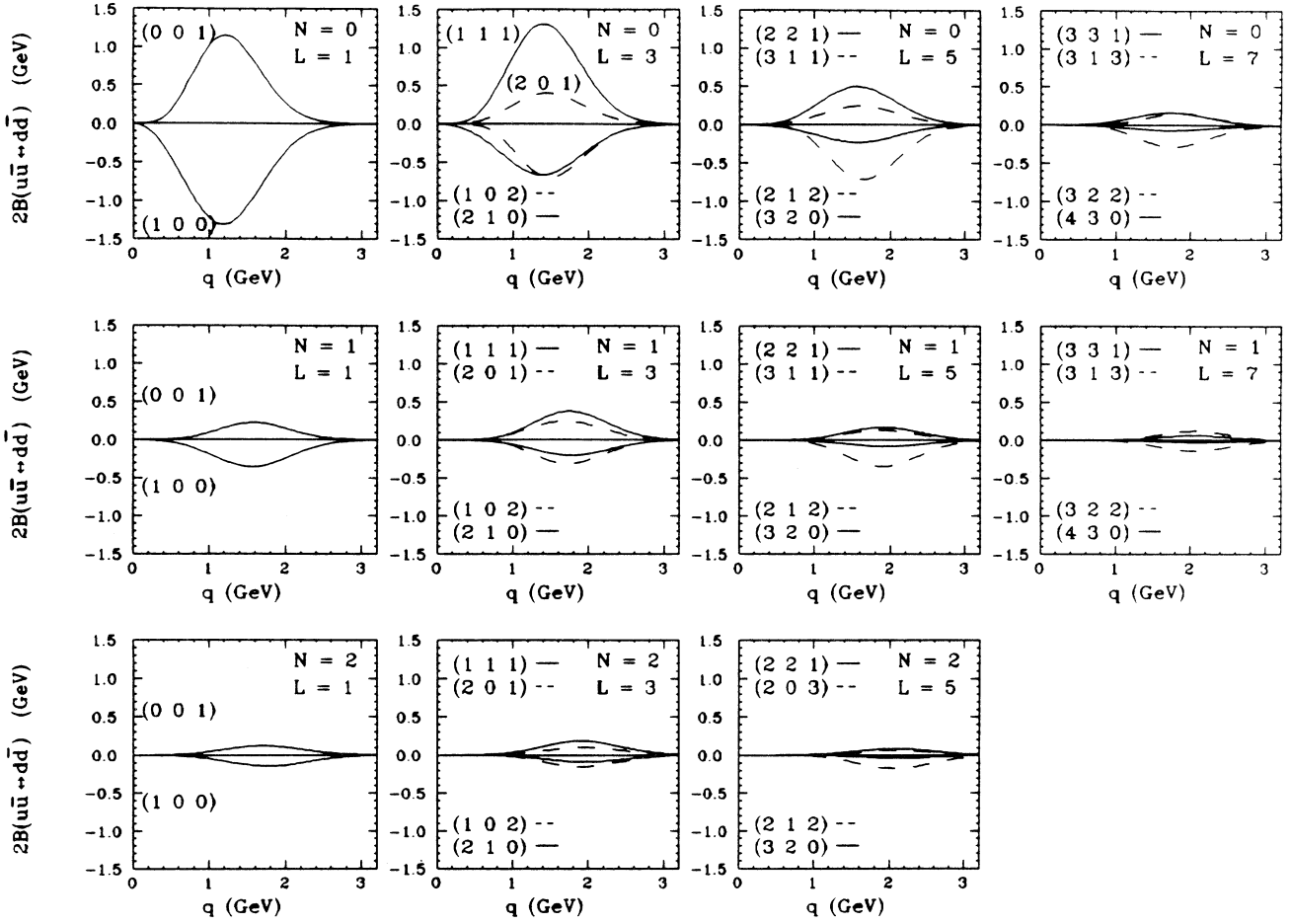
FIG. 3. The terms in the closure sum for B in Eq. (2) ordered by L \equiv l_B + l_C + l and N \equiv n_B + n_C - 2 , calculated using our canonical parameters \beta = 0.4 GeV, b = 0.18 GeV 2 , and r_q = 0.15 fm. The curves are labeled by (l_B, l_C, l) ; when l_B \neq l_C , (l_B, l_C, l) is an abbreviation for (l_B, l_C, l) + (l_C, l_B, l) . To avoid overcrowding on the graphs with L \geq 5 , we show only the “leading” terms, i.e., the ((L-1)/2, (L-1)/2, 1) and ((L+1)/2, (L-1)/2, 0) ones, and the two largest remaining terms.
