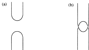
FIG. 1. A diagram associated with OZI rule violation shown in two time orderings.
