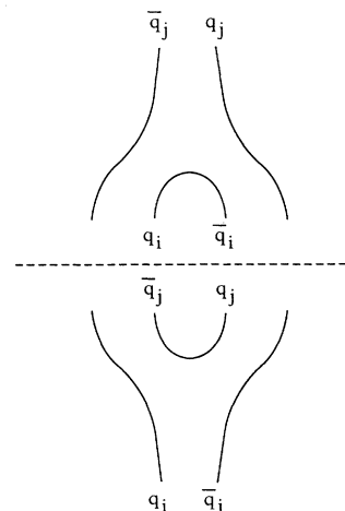
FIG. 2. OZI violation via two OZI-allowed amplitudes.
