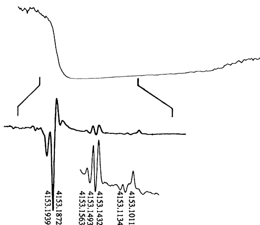
FIG. 3. Low-resolution spectrum (upper trace) and high-resolution spectrum (middle trace) of the Q_{1-0}(0) transitions. Part of the tone-burst spectrum is magnified in the bottom trace. The upper trace shows the entire exciton band. The sharp features appear at the high-frequency edge of this band. The frequency scan for the expanded central region is from 4152.64 to 4153.28 \text{ cm}^{-1} .
