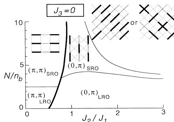
FIG. 1. Ground states of H for J_3=0 as a function of J_2/J_1 and N/n_b [ n_b=2S for \text{Sp}(1) \cong \text{SU}(2) ]. Thick (thin) lines denote first- (second-) order transitions at N=\infty . Phases are identified by the wave vectors at which they have magnetic long-range order (LRO) or short-range order (SRO). The links with Q_p \neq 0 in each SRO phase are shown. The large N/n_b , large J_2/J_1 has the two sublattices decoupled at N=\infty ; each sublattice has Néel-type SRO. Spin-Peierls order at finite N for odd n_b is illustrated by the thick, thin, and dotted lines. The (\pi, \pi) SRO and the “decoupled” states have line-type (Ref. 5) spin-Peierls order for n_b=2(\text{mod}4) and are VBS for n_b=0(\text{mod}4) . The (0, \pi) SRO state is a VBS for all even n_b .
