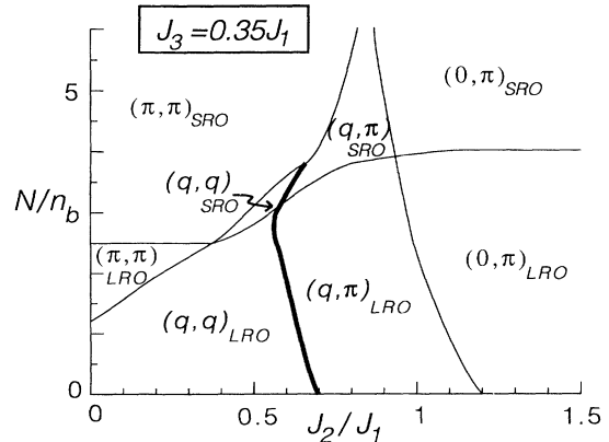
FIG. 3. As in Fig. 1 but for J_3/J_1 = 0.35 .
