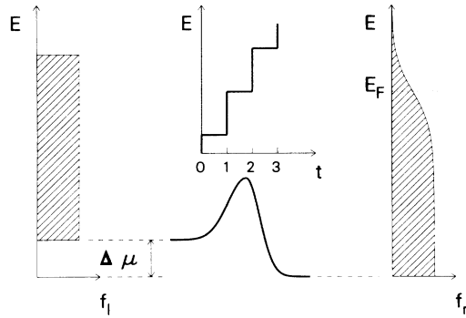
FIG. 3. Illustration of the origin of the transverse voltage. A cold 2DEG region on the left of the figure is connected via a quantum point contact to the current-heated channel region on the right-hand side. The solid line indicates the bottom of the conduction band in the point contact.
