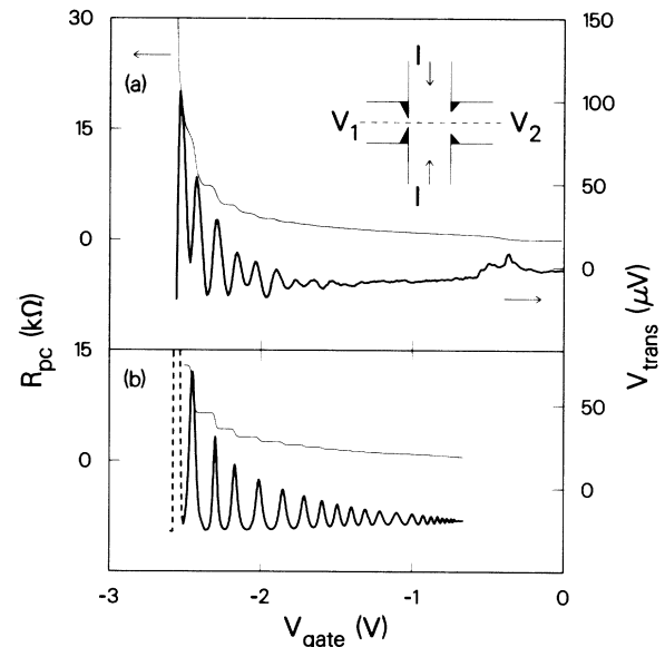
FIG. 1. (a) Experimental traces of V_{\text{trans}} (thick curve) and R_{\text{pc}} (thin curve) as a function of V_{\text{gate}} at lattice temperature T_0 = 1.65 K for I = 5 \mu\text{A} and V_{\text{gate}}^{\text{ref}} = -2.0 V. Inset: Arrangement for transverse-voltage measurements in a channel. The point-contact voltage probes are indicated in black. (b) Calculation of the transverse voltage (thick curve) using Eqs. (1)–(3) with electron temperature T = 4 K, T_0 = 1.65 K, and E_F = 13 meV. The thin curve gives the dependence of R_{\text{pc}} on V_{\text{gate}} , calculated for a temperature T_0 using experimental values of W and E_0 .
