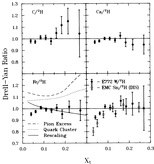
FIG. 3. Ratios of the Drell-Yan dimuon yield per nucleon, Y_A/Y_{{}^2H} , for positive x_F . The curves shown for Fe/{}^2H are predictions of various models of the EMC effect. Also shown are the DIS data for Sn/{}^2H from the EMC (Ref. 4).
