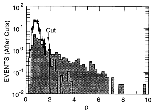
FIG. 1. Maximum isolation parameter \rho of all the tracks in an event for data (circles, with statistical errors), udscb QCD Monte Carlo simulation (solid line), and a 35\text{-GeV}/c^2 top quark (shaded area, normalized to data). The Monte Carlo simulation includes detector and beam background effects.
