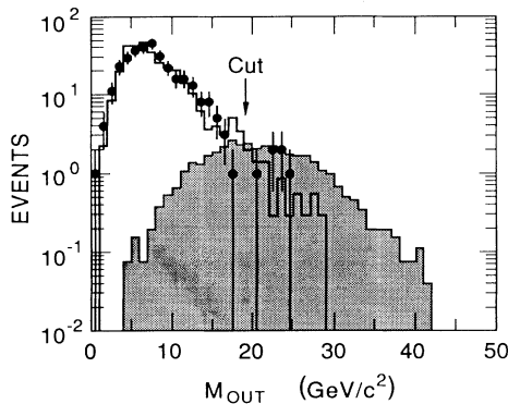
FIG. 4. Mass out of the event plane M_{\text{out}} for data (circles, with statistical errors), udscb QCD Monte Carlo simulation (solid line), and for a 35\text{-GeV}/c^2 b' quark decaying into cH^- (shaded area), with M_{H^-} = 25\text{ GeV}/c^2 and the H^- decaying 100% into c\bar{s} .
