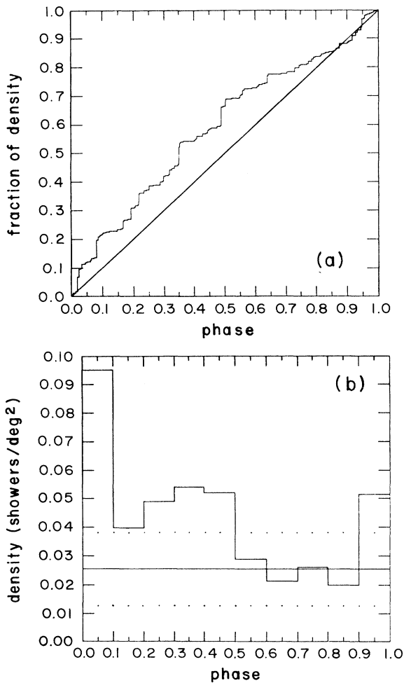
FIG. 3. (a) The full available information about the Cygnus X-3 4.8-h phase dependence by our plotting for each phase the fraction of the total density which arrived with lower phase values. The 45° line is the expected curve in the absence of periodicity. (b) The density which arrived in each of ten phase bins. The solid horizontal line shows the expected density (based on isotropic simulations), and the dotted lines indicate the rms deviation in the expected density for a single bin.
