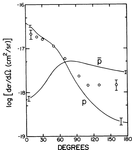
FIG. 2. He single-ionization cross sections singly differential in electron ejection angle. Solid lines: CTMC calculation. Data of Ref. 19.
