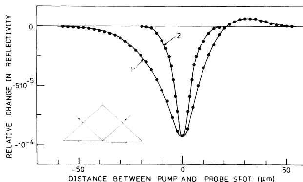
FIG. 1. Inset: Interaction region shown schematically. Two (almost) collinear beams, drawn here on top of each other, are focused through glass onto a 45-nm silver film. We measure changes in the reflectivity of the red probe pulse resulting from SP creation and decay by the yellow pump pulse. Main figure: This change shown as a function of position of both focused spots with respect to each other for a probe pulse arriving a few tens of picoseconds after the pump. Curve 1 displays the change in reflectivity for a displacement in the direction of propagation of the SP, whereas curve 2 shows the same effect for a perpendicular displacement.
