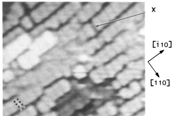
FIG. 2. A typical STM image of the GaAs(001) ( 2 \times 4 ) surface showing a 165 \times 130 \text{-}\text{\AA}^2 area including small islands one plane up (light) and one plane down (dark), each having the same structure as the main plane. Disorder in the pairing of arsenic atoms can be seen at X . The upper right-hand side of the image is a region of well-ordered ( 2 \times 4 ). The atom positions are marked with filled circles and the missing-atom sites are marked with open circles. The image was taken with the sample at -2.3\text{-V} and 0.2\text{-nA} tunneling currents. The gray scale covers a vertical height of 7 \text{\AA} .
