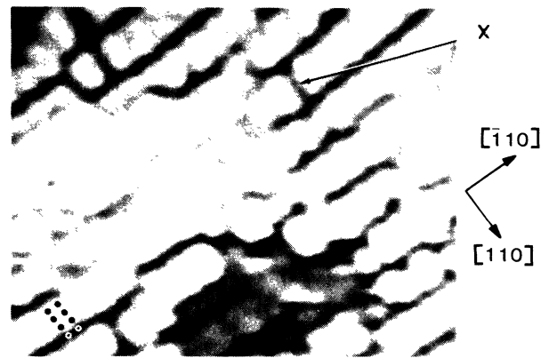
FIG. 2. A typical STM image of the GaAs(001) (2\times 4) surface showing a 165\times 130\text{-}\text{\AA}^2 area including small islands one plane up (light) and one plane down (dark), each having the same structure as the main plane. Disorder in the pairing of arsenic atoms can be seen at X. The upper right-hand side of the image is a region of well-ordered (2\times 4) . The atom positions are marked with filled circles and the missing-atom sites are marked with open circles. The image was taken with the sample at -2.3\text{-V} and 0.2\text{-nA} tunneling currents. The gray scale covers a vertical height of 7\text{ \AA} .
