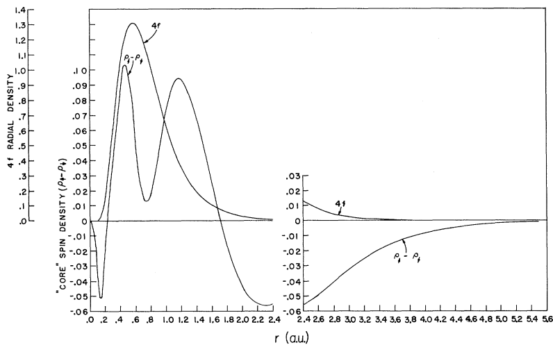
FIG. 1. The computed "core" electron spin density (\rho_{\uparrow} - \rho_{\downarrow}) for all the electrons other than the 4f shell and, for comparison, the 4f density as well. Note the change of scales at r = 2.4 a.u. to a common scale for both (\rho_{\uparrow} - \rho_{\downarrow}) and the 4f spin density.
