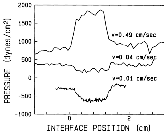
FIG. 1. Pressure across a 1.5-cm-long tube of porous medium as a function of position as nonwetting oil is displaced by wetting water at three different velocities. The jump in the pressure occurs as the interface moves through the porous medium, and reflects the magnitude of the capillary pressure.
