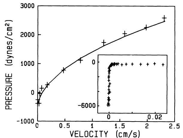
FIG. 2. Capillary pressure as a function of velocity. The solid line is a fit to the data. Inset: The large-pinning regime and the sudden jump in velocity which occurs upon depinning.
