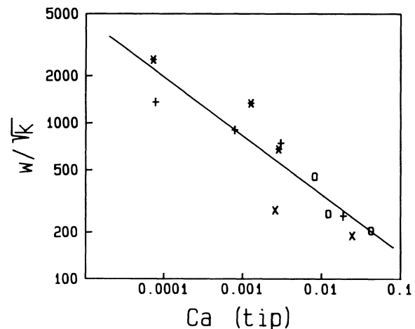
FIG. 3. Scaling behavior of the viscous-finger width in the wetting case, with the width normalized by \sqrt{\kappa} , and N_{Ca,t} the capillary number which refers to the velocity of the tip of the individual fingers. The slope of the solid line is -0.5 .
