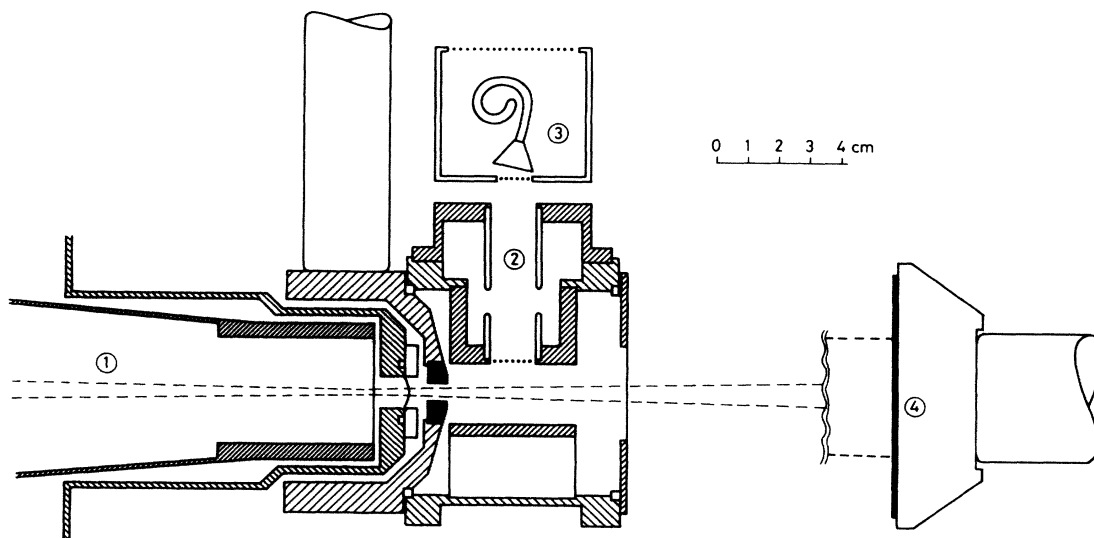
FIG. 1. Schematic drawing of the experimental setup. The dashed lines indicate the beam size (HWHM) for \sim 4.5 -MeV p^- . (1) LEAR vacuum. (2) Flight tube. (3) Channeltron detector. (4) End detector.
