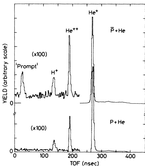
FIG. 2. Time-of-flight spectra obtained with \sim 4.5 -MeV p^- and p colliding with 3-mTorr He. The two spectra are normalized to the same He^+ yield.
