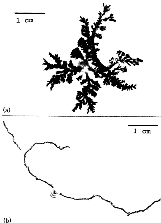
FIG. 3. (a) Open ramified deposit grown at high C and low \Delta V ( C = 1M , \Delta V = 2 V). (b) Stringy pattern grown at higher \Delta V ( C = 0.01M , \Delta V = 12 V).
