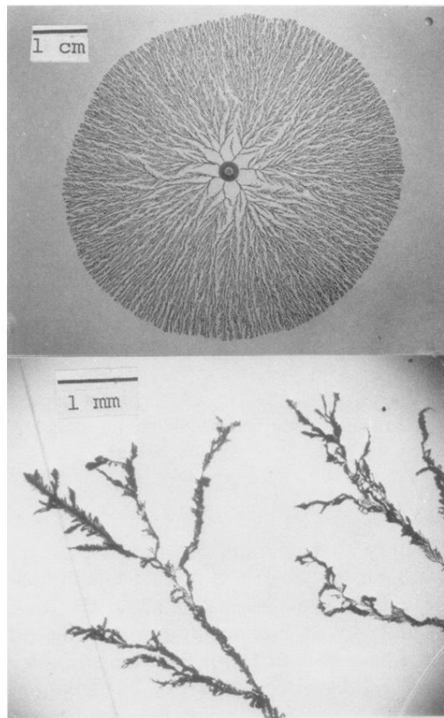
FIG. 2. Homogeneous pattern produced by the tip-splitting instability, at two different magnifications ( C = 0.01M , \Delta V = 6 V).
