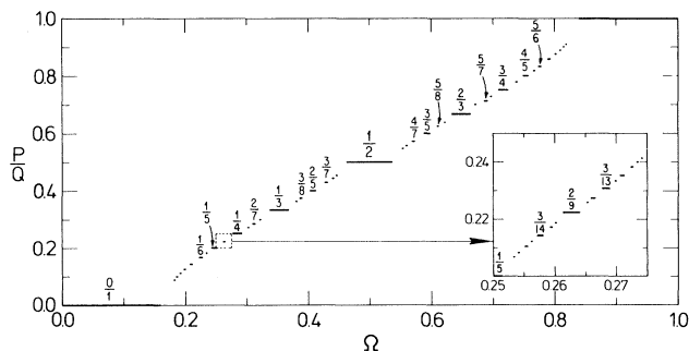
FIG. 1. The mode-locking structure at K = 1 for the map (1). The "devil's staircase" is complete, and the complement of the mode-locked windings is of Lebesgue measure zero and universal fractal dimension D (Ref. 3).
