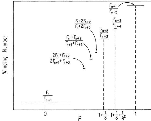
FIG. 2. The universal "devil's staircase" as generated from the unstable manifold. Locked ranges denoted by a thin line can be obtained directly from the stability of g_p(x) . The locked ranges shown by thick lines are obtained by composing the universal objects. The notation F_n/F_{n+1} is arbitrary in the sense that n is "very high." In fact, we use the notation [0] for F_n/F_{n+1} , [1] for F_{n+1}/F_{n+2} , etc. (Ref. 11).
