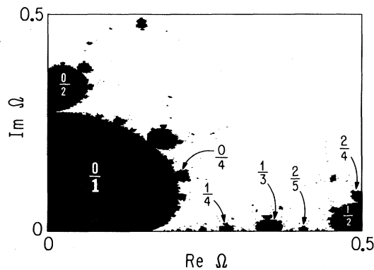
FIG. 3. Mode locking in the complexified circle map. Plotted is the complex \Omega plane and in the black regions the iterations are mode locked. The real axis has the same structure as Fig. 1.
