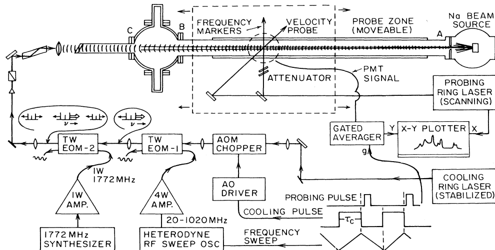
FIG. 2. Schematic of two-laser-atom-beam cooling experiment. The cooling-laser output is fed through an acousto-optic shutter, a \text{LiTaO}_3 traveling-wave electro-optic modulator (TW EOM) which puts on the frequency-swept sidebands, and an additional TW EOM to provide the F=1 atom recovery sideband. The sigma-polarized 35-mW cooling-laser beam is carefully "mode matched" to the weakly diverging atomic beam (3 mrad full angle). After the sweep, the cooling-laser beam is cut off and we briefly sample the fluorescence induced by the slowly scanning weak ( 100 \mu\text{W} ) probe laser, thus measuring the resultant velocity distribution as a function of time (and axial position). A 3.5\text{-}\mu\text{W} transverse probe beam provides frequency markers for the probe scan.
