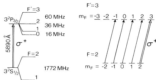
FIG. 1. Level scheme of Na with the cooling transitions.
