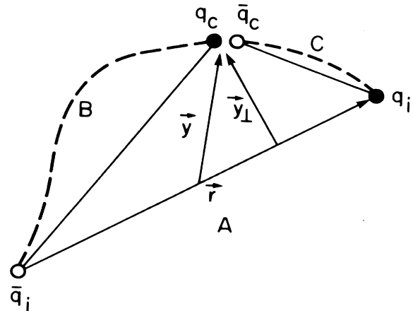
FIG. 1. The geometry of string breaking showing the initial meson separation \mathbf{r} = \mathbf{r}_{q_i} - \mathbf{r}_{\bar{q}_i} and the pair creation vector \mathbf{y} = \frac{1}{4}(\mathbf{r}_{q_c} + \mathbf{r}_{\bar{q}_c} - \mathbf{r}_{q_i} - \mathbf{r}_{\bar{q}_i}) ; the dashed line represents the (newly broken) string.
