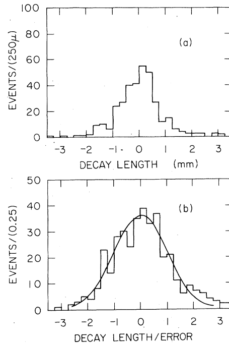
FIG. 2. (a) Measured decay lengths for "pseudo- \tau " decays; (b) decay length divided by its calculated error for pseudo- \tau decays. The solid curve is a unit-width Gaussian function, normalized to the data between -2.5 \leq l/\sigma \leq 2.5 .
