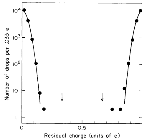
FIG. 2. Distribution of residual charge for all of our water drops. The curve is a fitted Gaussian with a standard deviation 0.037e .
