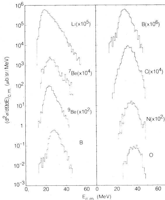
FIG. 2. Energy spectra in the c.m. system for various ejectiles detected at \theta_{c.m.} = 171^\circ . Before correction for carbon contamination the lower level threshold varied from 4 to 12 MeV in the c.m. for Li to O ejectiles, respectively.
