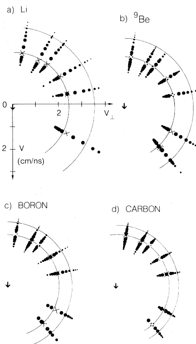
FIG. 1. Invariant cross-section plots ( \propto V^{-2} d^2\sigma/d\Omega dV ) for representative ejectiles (Li, ^9\text{Be} , B, and C). The diameter of the dots is proportional to the logarithm of the cross section and the \times 's indicate the peak of velocity distribution. The two large arcs are sections of circles centered on the c.m. velocity (center arrow) appropriate for complete fusion. The beam direction ( 0^\circ ) is indicated by the c.m. velocity vector.
