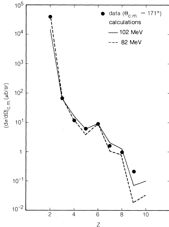
FIG. 3. Experimental (circles) and theoretical yields vs ejectile atomic number ( Z ).
