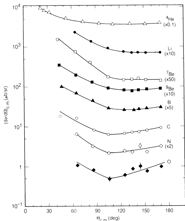
FIG. 4. Angular distributions in the c.m. system for various ejectiles. The curves through the data points are to guide the eye. Statistical error bars are only shown when they exceed the size of the data points.
