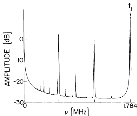
FIG. 7. Period tripling.
