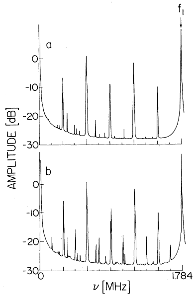
FIG. 8. (a) and (b) Period tripling with additional period doubling.
