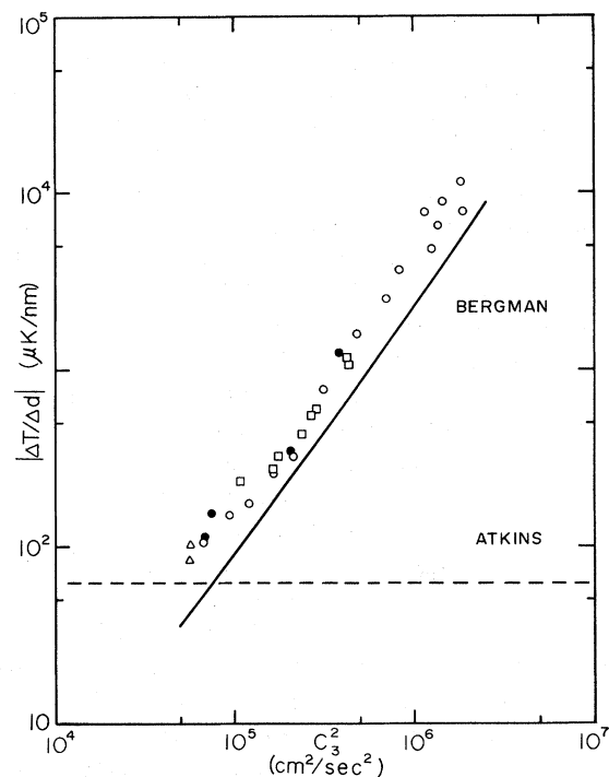
FIG. 3. Magnitude of the relative amplitude of the temperature oscillation to the thickness oscillation at 1.35 K vs the square of the observed third-sound velocity. The various symbols correspond to various experimental runs with \nu = 1 kHz. Near |\Delta T/\Delta d| values of 10^3 \mu\text{K}/\text{nm} we expect that our calibration errors are about \pm 20\% . At the extremes of the data these errors may be as much as a factor of 2 larger.
