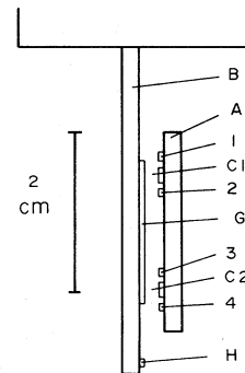
FIG. 1. Schematic representation of the apparatus. The glass plates A and B extend 2.5 cm into the page. The plate spacing and the size of the evaporated strips has been exaggerated for clarity. Strips 1-4 are superconducting bolometers, H is a heater and G a ground plane which serves as one plate of capacitors C1 and C2. Not shown are the epoxy beads which maintain the separation. The assembly is suspended from the base of a recirculating ^3\text{He} refrigerator which was not used for the measurements described here.
