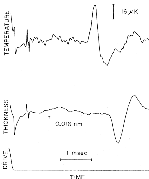
FIG. 2. Bolometer (top) and capacitor (middle) response to a \nu = 3 kHz drive pulse (only half of which is displayed). The capacitor signal is displaced to the right because the capacitor is farther downstream from the driver than is the bolometer. Here T = 1.30 K and the film thickness d \approx 13 layers.
