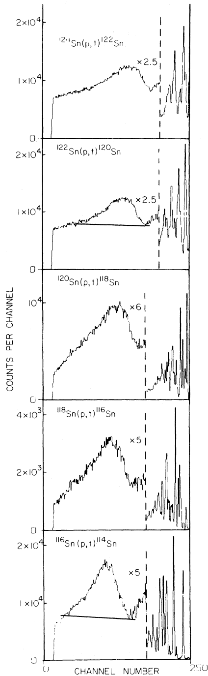
FIG. 1. Triton spectra from the (p,t) reaction on some even-even isotopes of tin at a laboratory angle of 16^\circ . The proton bombarding energy was 42 MeV. The absolute energy scale is the same for all of the spectra. The solid straight lines in the ^{116}\text{Sn}(p,t)^{114}\text{Sn} and ^{122}\text{Sn}(p,t)^{120}\text{Sn} spectra show the background subtracted in determining the cross section.
