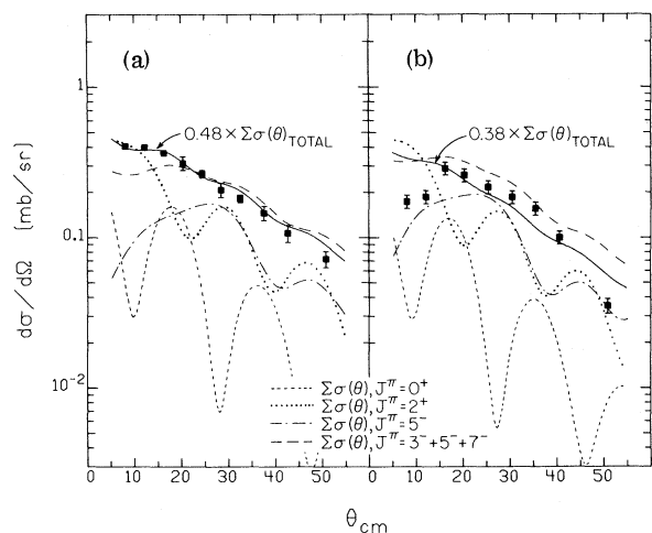
FIG. 2. Angular distribution for (a) ^{116}\text{Sn}(p,t)^{114}\text{Sn} and (b) ^{122}\text{Sn}(p,t)^{120}\text{Sn} for the "peak" in the triton spectrum at an excitation energy of about 8 MeV. The curves are DWBA calculations as outlined in the key. Only the total predicted cross section (solid curve) has been normalized to the data.
