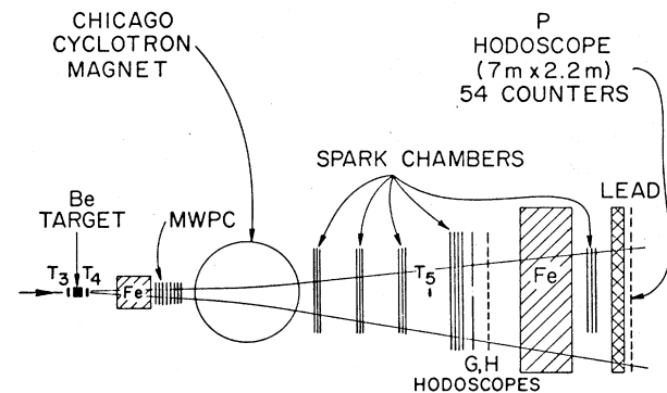
FIG. 1. The spectrometer.
