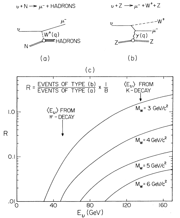
FIG. 1. (a) Deep-inelastic neutrino scattering, mediated by the hypothetical W . (b) W^+ production (a similar diagram with the W - N interaction has been omitted). (c) The predicted ratio of observed events of type (b) to type (a) as a function of neutrino energy and W mass. The detection efficiency of the apparatus, the W^+ production cross section, and the \mu^- production cross section with W propagator are all included.
