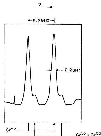
FIG. 2. Fabry-Perot analysis of tungsten-lamp-excited R_1 fluorescent spectrum of Czochralski ruby (0.05 wt% \text{Cr}_2\text{O}_3 at 4.2°K. Interorder separation of 11.5 GHz equals the R_1 splitting. The instrument linewidth is \sim 0.2 GHz.
