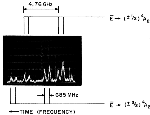
FIG. 3. Oscillogram of Fabry-Perot analyzed laser-induced fluorescence of the ruby R_1 line at 4.2^\circ\text{K} . Sweep speed is 1 msec/cm.
