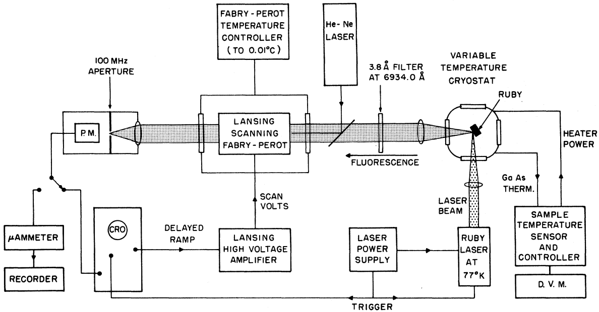
FIG. 1. Schematic of apparatus used for line-narrowing experiments.
