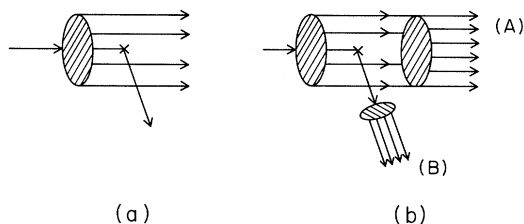
FIG. 1. Deep inelastic scattering of an incident proton by a current interacting at X . All the initial and final-state interactions illustrated by the blobs in diagram (b) in the Bjorken limit reduce to (a) in the parton model.
