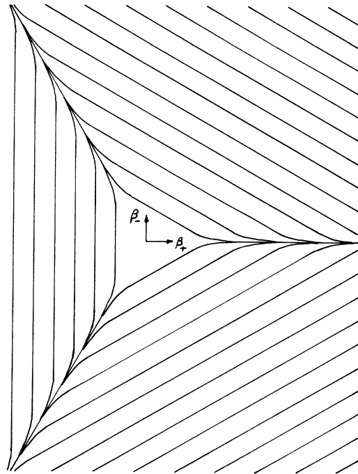
FIG. 1. Equipotentials of the function V(\beta) are sketched here in the \beta plane from the asymptotic forms of Eqs. (9) and (10). (Equipotentials near the origin, not shown, are closed curves for V < 1 .) Between successive equipotentials on this diagram, which have separations \Delta\beta = 2 , V increases by a factor of e^8 \approx 3 \times 10^3 . From Eq. (5), the system point \beta(\Omega) moves with velocity |d\beta/d\Omega| = 2 except when it approaches a limiting equipotential V = \Lambda e^{4\Omega} . This limiting equipotential moves outward with velocity |d\beta_{\text{wall}}/d\Omega| = 1 except during the brief period when the system point \beta bounces against it. The "velocity" d\beta/d\Omega changes its direction in what appears to be an ergodic way as a result of these bounces; and whenever it is closely parallel to one of the three corner axes, horizons along the corresponding one of the three expansion axes of the universe approach (or perhaps exceed) the circumference of the universe.
