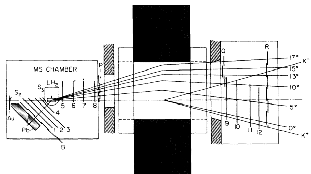
FIG. 1. The experimental apparatus drawn to scale. MS_{1-4} , MS_{5-8} and MS_{9-12} are digitized wire spark chambers. Arrays B , P , and R are the triggering counters. Typical trajectories through the system are shown.
