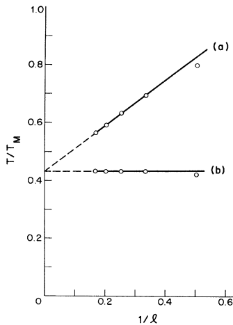
FIG. 2. The plane triangular lattice ( z=6 ) with S=\frac{3}{2} . (a) The ratios a_l/a_1 a_{l-1} approach T_c/T_M \cong 0.435 . (b) The function t_l(\gamma'=2.75) . As in Fig. 1, the coefficients a_l were obtained from the general expressions of Rushbrooke and Wood, 1 valid for any spin and lattice.
