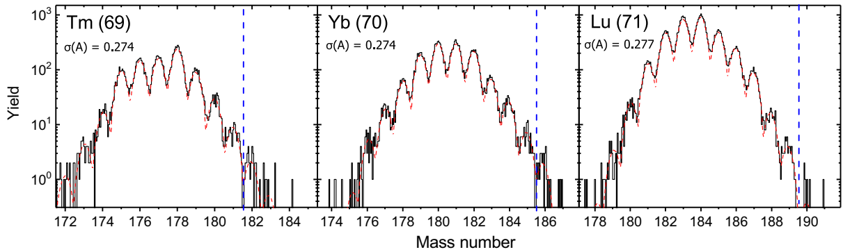
FIG. 5. Mass spectra of elements with atomic numbers ranging from 69 to 71 obtained with the new-isotope-search settings of the separator. A gate condition on Z with a width [Z - 0.3, Z + 0.3] was applied to generate these spectra in addition to the selection of the heliumlike charge state (see Fig. 3). The standard deviation obtained for Gaussian functions having a constant width (dashed red lines) is indicated for each element. The dashed blue line marks the limit of known isotopes for each element.
