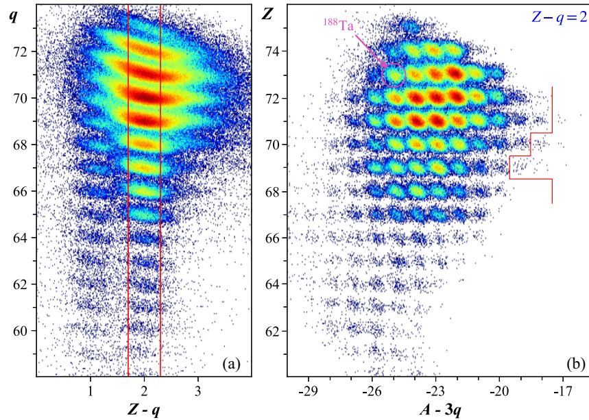
FIG. 3. (a) The separation of charge states is demonstrated in the q vs Z-q spectrum of a setting optimized to observe ^{186}\text{Yb}^{68+} ions, in which the heliumlike charge states were most prominent. A charge-state selection gate [1.7 to 2.3] on the heliumlike ions was applied to obtain the spectrum in (b), with the Z distribution of the heliumlike ions as a function of (A/q - 3) \times q , where the mass-to-charge ratio, A/q , was constructed from TOF and B\rho measurements. This PID plot, labeled as Z vs A - 3q , demonstrates the quality of the mass, charge, and elemental separation. The limit of previously observed nuclei is indicated by the solid red line. A \gamma -ray spectrum observed in coincidence with the labeled ^{188}\text{Ta}^{71+} ions was used to confirm its identification (see text).
