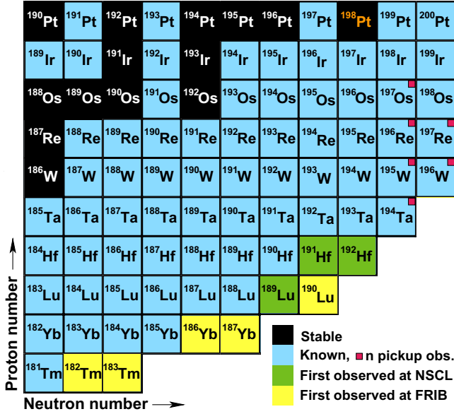
FIG. 1. Region of the nuclear chart, 69 \leq Z \leq 78 and 112 \leq N \leq 122 , showing the known nuclei and the eight nuclides that were recently discovered at NSCL [11] and FRIB (present work) by the fragmentation of ^{198}\text{Pt} beams. Previously known isotopes observed in the present work whose formation involved one- and two-neutron pickup relative to the projectile are marked.
