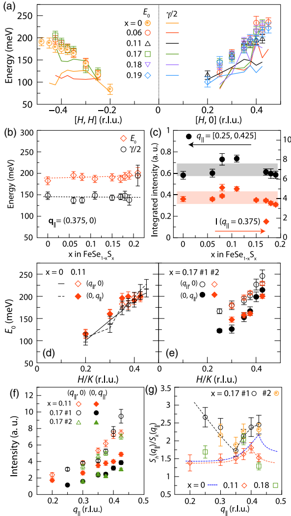
FIG. 3. (a) E_0 and \gamma/2 of the spin excitations along H [ S_h(q_{||}, E) ] and [H, H] [ S_{hh}(q_{||}, E) ] for unstrained x = 0, 0.06, 0.11, 0.17, 0.18 , and 0.19 . (b) E_0 and \gamma/2 of the spin excitation at H = 0.375 of unstrained samples as a function of the doping level x . (c) Doping dependence of the spin-excitation intensity S_h(q_{||}) for q_{||} = 0.375 (red diamonds) and the momentum integrated S_h(q_{||}) in the momentum range q_{||} = [0.25, 0.425] (black circles). (d), (e) Comparison of E_0(q_{||}) between S_h(q_{||}, E) and S_k(q_{||}, E) for (d) x = 0 (black lines), 0.11 (red diamonds), and (e) x = 0.17 . (f) Energy-integrated spin-excitation intensity S_h(q_{||}) (open symbols) and S_k(q_{||}) (filled symbols) for x = 0.11 (red diamonds), 0.17 (sample 1) (black circles), and 0.17 (sample 2) (green triangles). (g) Doping-dependent spin-excitation anisotropy \phi(q_{||}) = S_h(q_{||})/S_k(q_{||}) for x = 0 (blue dashed curve), 0.11 (red diamonds), 0.17 (black and illuminated orange circles), and 0.18 (green squares). The red and black dashed curves are guides to the eyes.
