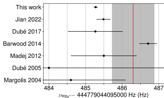
FIG. 4. Results of measurements of the ^{88}\text{Sr}^+ clock transition frequency obtained in the previous Refs. [21,39–43] and this Letter. The recommended value for \nu^{88\text{Sr}^+} as a secondary representation of the second approved in 2021 [44] is shown by the red line, and the shaded area is its uncertainty.
