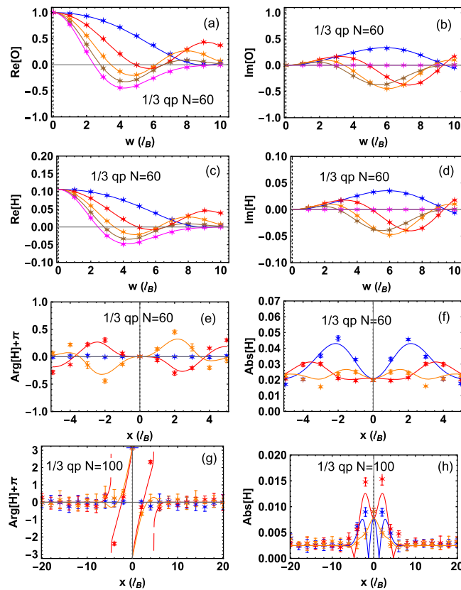
FIG. 2. Same as Fig. 1 in the original Letter but for the quasiparticle of \nu = 1/3 .
