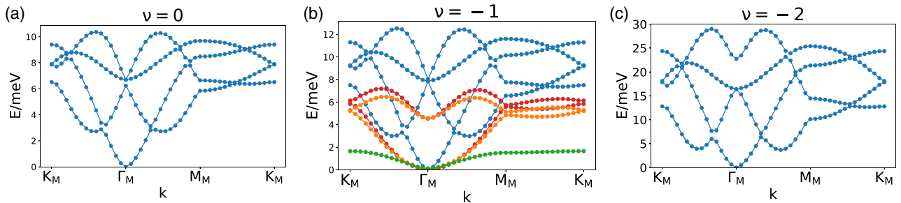
FIG. 2. Excitation spectrum at \nu = 0, -1, -2 . Blue, orange, red, and green denote the fluctuations in the full-empty sector, half-empty sector, full-half sector, and half-half sector, respectively.
