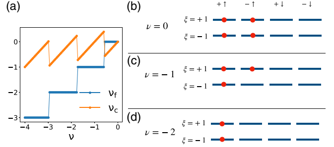
FIG. 1. (a) Filling of f electrons ( \nu_f ) and c electrons ( \nu_c ) as a function of total filling ( \nu ) in the zero hybridization model. Three transition points are \nu \sim -0.59, -1.73, -2.95 (b),(c),(d). Illustrations of ground states at \nu = 0, -1, -2 . The red dot means the filling of one f electron.
