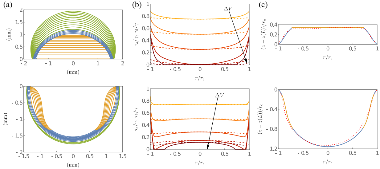
FIG. 3. (a) Theoretical predictions of the droplet profiles during evaporation of a sessile (top, V_i = 13.05 \text{ mm}^3 , C = 2 \text{ } \mu\text{mol L}^{-1} , \text{Bo} = 0.99 ) and a pendant droplet (bottom, V_i = 7.77 \text{ mm}^3 , C = 4 \text{ } \mu\text{mol L}^{-1} , \text{Bo} = -0.70 ). The green solid curves are obtained from the fluid equation (2), which remains valid while the bulk concentration C < C_e ; while for C \geq C_e the elastic equations (3), (4) are solved. Blue and orange solid curves indicate the elastic regions and wrinkled or crumpled regions of the interface, respectively. (b) Dimensionless meridional (dashed curves) and hoop stress (solid curves) versus the dimensionless radial position r/r_c at different volumes V ( V = 3.57, 4.91, 5.26, 5.60, 5.93 \text{ mm}^3 for the sessile droplet, while V = 5.77, 6.15, 6.43, 6.76, 7.10 \text{ mm}^3 for the pendant droplet), the arrows indicate the direction of increasing evaporated volume \Delta V . (c) Predicted (solid curves) and experimental droplet profiles (dotted curves) at a given time for a sessile (top, V = 3.57 \text{ mm}^3 ) and a pendant droplet (bottom, V = 5.77 \text{ mm}^3 ). Here, color shows the predicted wrinkled or crumpled (yellow), or tensile (blue) regions.
