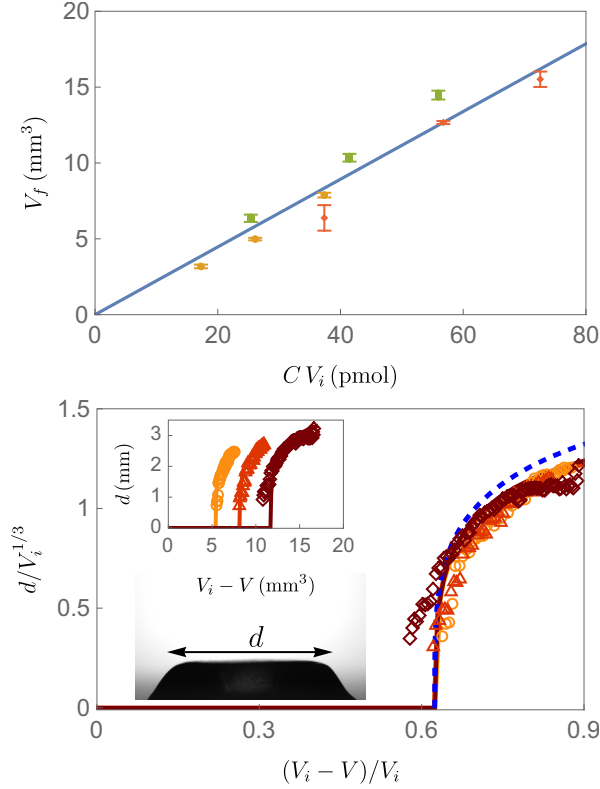
FIG. 2. Top: experimental data for the droplet volume V_f at which sessile droplets start to flatten as a function of the total number of HFBI molecules contained in the droplet (the product of initial concentration C and initial droplet volume V_i ). The orange, green, and red dots represent the data for C = 2, 3, 4 \mu\text{mol L}^{-1} , respectively. The blue solid line shows the linear fit of the experimental data. (Bottom) The diameter d of the flat spot increases with the volume of liquid lost to evaporation, V_i - V . Raw measurements for droplets with C = 2 \mu\text{mol L}^{-1} and V_i = 8.63, 13.05, 18.68 \text{ mm}^3 (orange, red, and brown, respectively) shown in the inset collapse onto a master curve when lengths are rescaled by V_i^{1/3} . The blue dashed curve shows the prediction of a purely geometrical model, see Eq. (S22) in Supplemental Material [23].
