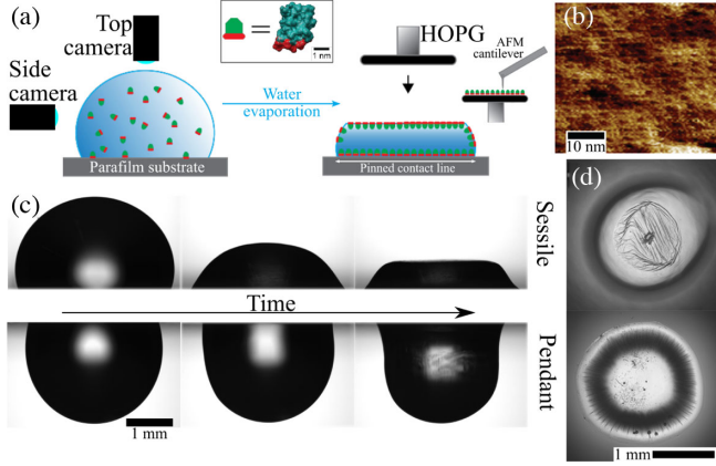
FIG. 1. (a) Sketch of the experimental setup. A droplet is placed on a Parafilm substrate and its shape is recorded from above and the side by cameras. After the formation of the flattened region, a highly ordered pyrolytic graphite (HOPG) substrate was brought in contact with the top of the droplet to perform imaging through an atomic force microscope (AFM). (b) AFM image of HFBI monolayer at the air-water surface. (c) Sessile (top) and pendant (bottom) droplet shapes at different times during evaporation. The initial volume is V_i = 13.1 \text{ mm}^3 in both cases, while the initial concentration of HFBI 2 \mu\text{mol L}^{-1} for the sessile drop and 4 \mu\text{mol L}^{-1} for the pendant drop. (d) Plan views of a crumpled sessile (top) and a wrinkled pendant (bottom) droplet.
