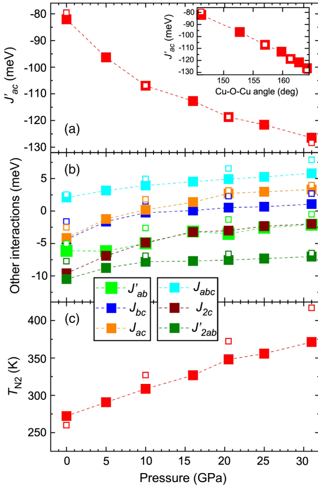
FIG. 4. Pressure dependence of (a) J'_{ac} , (b) J'_{ab} , J_{bc} , J_{ac} , J_{abc} , J_{2c} , and J'_{2ab} , and (c) T_{N2} . Closed and open symbols show the results of the LMTO and QE calculations, respectively. The notations for the parameters are shown in Fig. 3. The inset in (a) shows the dependence of J'_{ac} on the angle Cu-O-Cu.
