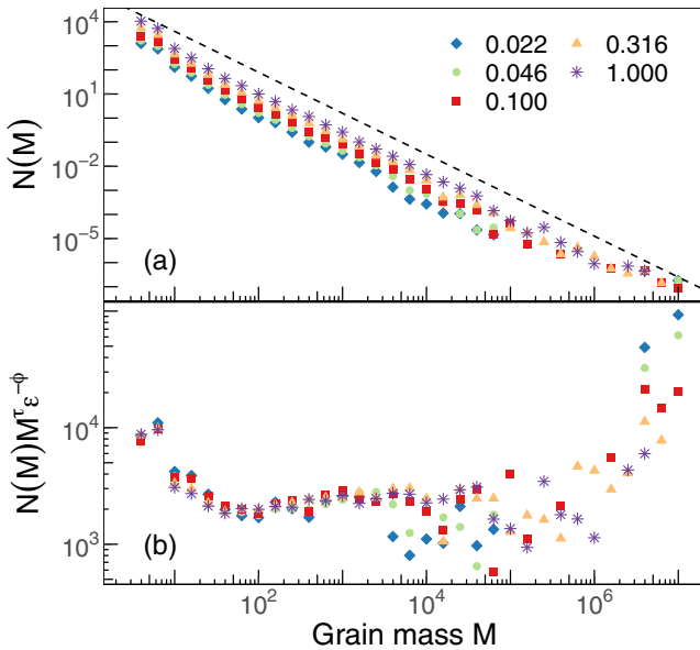
FIG. 2. (a) Quasistatic distributions N(M) at the indicated strains \epsilon . The dashed line represents a power law with exponent \tau . (b) N(M) scaled by the measured power law and e^\phi . Values of exponents are listed in Table I.
