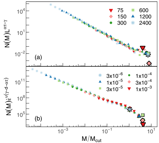
FIG. 8. (a) Collapsed QS distributions from Fig. 4 for M > M_{\text{min}} using the procedure in Eq. (1) and a value of M_{\text{cut}} = L^\alpha . (b) Similarly collapsed FR distributions from Fig. 3(b) using Eq. (2) and M_{\text{cut}} = \dot{\epsilon}^{-\nu\alpha} . Exponents are taken from Table I. The largest mass of each dataset is enlarged for visibility.
