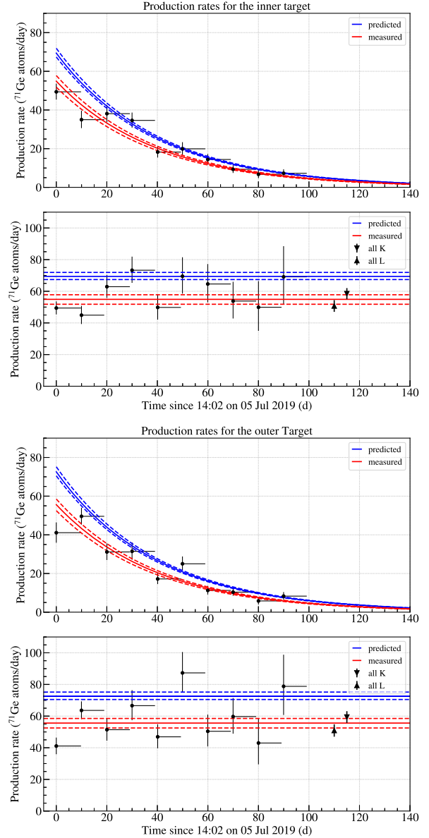
FIG. 2. Top: the measured K + L peak rates of the inner target volume. Middle, top: normalizes the production rate to the reference time, the combined results for events in the L and K peaks are shown. The blue (red) region represents the predicted (measured) production rate. Middle, bottom: similar to the top panel but for the outer volume. Bottom: similar to the middle-top panel but for the outer volume. The dotted lines enclose the \pm 1\sigma uncertainty regions. For all panels, the horizontal lines indicate the exposure duration with the likelihood fit results plotted at the start of exposure.
