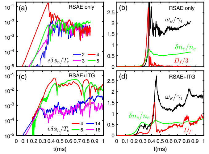
FIG. 1. Time history of perturbed electrostatic potentials e\delta\phi/T_e for RSAE ( n = 2 - 5 ) from simulation of RSAE only [panel (a)] and for ITG ( n = 14, 16 ) from simulation of ITG-RSAE [panel (c)]. Corresponding zonal flow shearing rate \omega_E/\gamma_4 , electron density perturbation \delta n_e/n_e (%), and effective EP diffusivity D_f (m 2 /s) are shown in panel (b) and panel (d).
