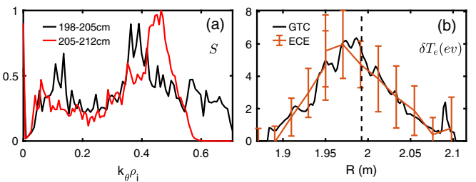
FIG. 3. Spectrum S of electron density perturbation \delta n_e as a function of poloidal wave number k_{\theta}\rho_i in two radial regions [panel (a)], and radial profiles of electron temperature perturbation \delta T_e [panel (b)] from GTC simulations and ECE measurements in DIII-D.
