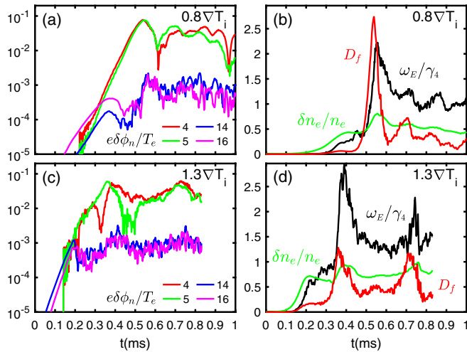
FIG. 4. Time history of perturbed electrostatic potentials e\delta\phi/T_e for RSAE ( n = 4, 5 ), and ITG ( n = 14, 16 ) from simulations with a weaker [panel (a) using 0.8\nabla T_i ] or stronger [panel (c) using 1.3\nabla T_i ] thermal ion temperature gradient. Corresponding zonal flow shearing rate \omega_E/\gamma_4 , electron density perturbation \delta n_e/n_e (%), and effective EP diffusivity D_f (m 2 /s) are shown in panels (b) and (d).
