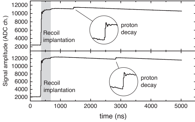
FIG. 1. Two examples of a wave form recorded for the fast proton decay of ^{149}\text{Lu} . The grey region marks a dead time set in software.
