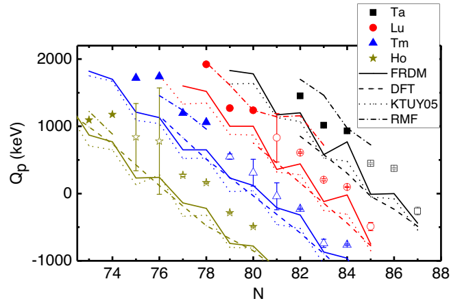
FIG. 4. Proton-decay Q value of selected tantalum (black), lutetium (red), thulium (blue), and holmium (olive green) nuclei. Experimental data for nuclei with a known proton-decay branch are indicated with solid symbols (this work and Ref. [12]), whereas open symbols denote other nuclei [47]. The lines show the predictions of different state-of-the-art theoretical models, namely, finite-range droplet model (solid line, [31]), energy-density functional theories [48] (dashed line, average of six models based on SkM* [49], SkP [50], SLy4 [51], SV-min [52], UNEDF0 [53], and UNEDF1 [54] functionals), KTUY05 atomic mass model (dotted line [55]), and the deformed relativistic mean field theory (dash-dotted line, [32]).
