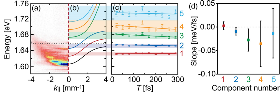
FIG. 3. (a) Energy-momentum-resolved PL map (for negative k_{||} , see Supplemental Material [20] for the full dataset). (b) Simulated polariton dispersion relations using the vibronic polariton model. The horizontal dotted line indicates the energy of pure excitons. (c) Retrieved energy positions (squares) of five bands as functions of T , and linear fitting results (solid lines). The error bars are evaluated as the standard deviation of the fluctuations calculated from the differences between the measured values (squares) and linear fit results (solid lines) at each T . Colored shaded areas in (b) and (c) indicate the total confidence ranges of experimentally determined energy positions from 2D spectroscopy data evaluated over all T , to facilitate comparison with the theoretical dispersion curves. (d) Linear slopes of the five fits from (c), with error bars depicting 95% confidence bounds from the fit.
