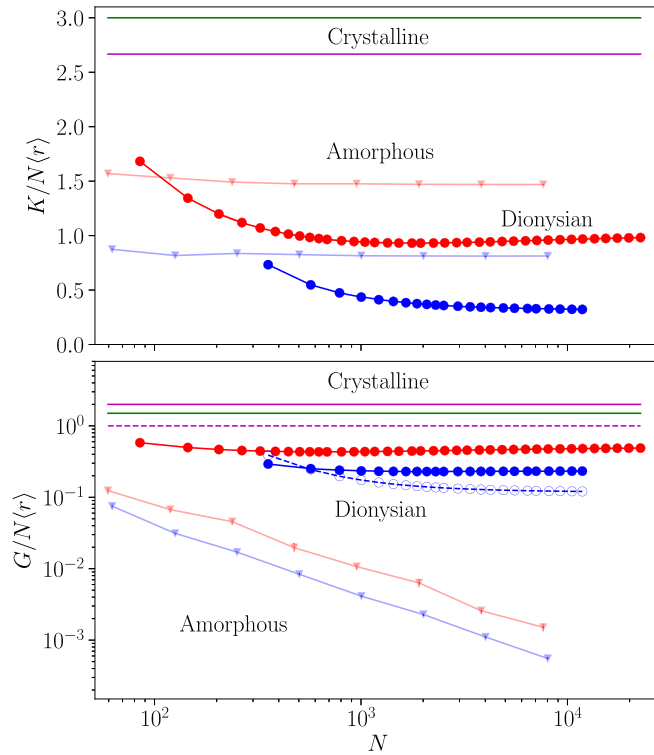
FIG. 3. The dimensionless bulk K and shear G moduli per sphere for Dionysian and amorphous packings in a unit cell as a function of the number of spheres N . The green line represents a two dimensional triangular packing, the magenta line represents a three dimensional FCC packing, and red and blue represent two dimensional and three dimensional packings, respectively. The dashed curves with open symbols represent G_{110} , the shear modulus in direction (1,1,0), whereas the solid curves with closed symbols represent G_{100} . The results are exact for the Dionysian packings and crystals. For the amorphous systems, sufficiently many systems were sampled to make the standard error bars smaller than the plot markers. In the limit of large N , the bulk modulus per sphere asymptotes to a positive value in two and three dimensions for all of the systems. The shear modulus for crystals and Dionysian packings plateaus for large N indicating that these remain very stiff. On the other hand, the amorphous packings have a shear modulus that decreases like 1/N [22].
