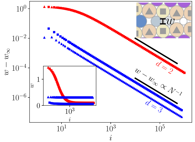
FIG. 2. Top right inset: demonstration of the definition of a gap for a circle. The b circles, indexed by i , oscillate in size and are separated into two categories labeled by squares and triangles. Bottom left inset: The gap value for both square and triangular marked spheres asymptotes in two and three dimensions. When the asymptotic gap value is subtracted, the gap sizes follow a power law of N^{-1} as they reach their respective asymptotic values.
