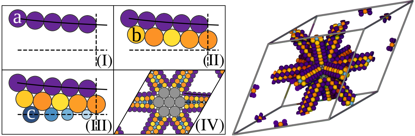
FIG. 1. The construction of a Dionysian packing in two and three dimensions. Left: (I) A row of n = 5 circles a (purple) lie on a strictly convex curve \mathcal{C} such that each circle kissing its neighbors. (II) A row of n = 5 circles b (orange and yellow) are placed such that they kiss two circles a from below and a circle b on either side. The rightmost b circle is constrained such that its center lies on the vertical line tangent to the rightmost a circle. (III) A row of n - 1 = 4 circles c (blue) lie on a horizontal line and kiss two b circles above. (IV) A bridge is formed by reflecting the circles about the dotted lines of symmetry. Three bridges are combined and their centers are filled as shown (gray). Because of the periodic boundary conditions, each of the bridges wraps around the unit cell to contact the central gray spheres twice such that each unit cell contains six half-bridges or three full bridges. The resulting packing, which is jammed and shear stable, has a very low density and is a Dionysian packing in the limit as n \rightarrow \infty . Right: A three dimensional mechanically stable packing at arbitrarily low densities. Such a construction contains the same three types of spheres as in the two dimensional analog but with additional symmetries and an entirely unrelated set of spheres filling the void region (gray). The three dimensional Dionysian packing has a much narrower set of convex curves \mathcal{C} for which overlaps do not occur (as detailed in the Supplemental Material [16]). This requires a much more subtle curvature of \mathcal{C} which is not apparent to the naked eye in this figure.
