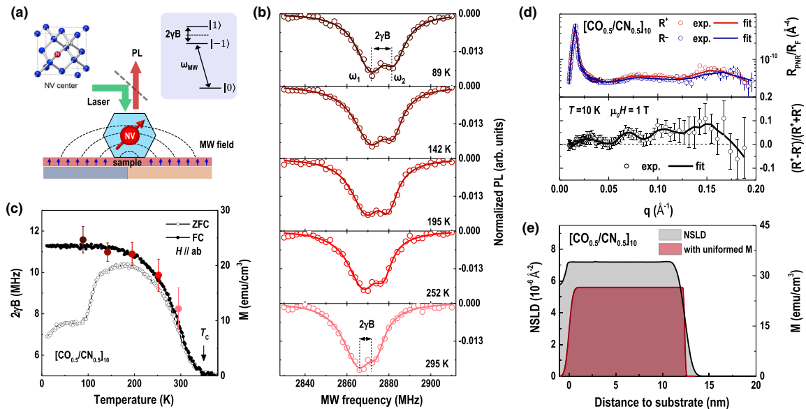
FIG. 3. Nanoscale magnetic probing using NV spins in nanodiamond and PNR. (a) Schematic of diamond NV-based magnetometry. (b) Zero-field optically detected magnetic resonance (ODMR) spectra of ensemble NV centers in a nanodiamond on the surface of [\text{CO}_{0.5}/\text{CN}_{0.5}]_{10} SL at various temperatures. (c) M - T curves of [\text{CO}_{0.5}/\text{CN}_{0.5}]_{10} at 1 kOe after zero-field cooling (open circles) and field cooling of 1 kOe (solid circles). The temperature dependence of 2\gamma B is plotted as color circles for comparison. (d) Normalized neutron reflectivities (upper panel) from both spin-up and spin-down neutrons and spin asymmetry (lower panel) of [\text{CO}_{0.5}/\text{CN}_{0.5}]_{10} SL as a function of \vec{q} . (e) Magnetization depth profile calculated from the fitted neutron magnetic scattering length density (NSLD).
