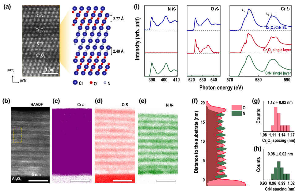
FIG. 1. Structural and electronic characterization of \text{Cr}_2\text{O}_3/\text{CrN} SLs. (a) A highly-magnified STEM image from a region marked with an orange dashed rectangle in (b), which is a cross-sectional STEM-HAADF image for a [\text{CO}_1/\text{CN}_1]_{10} SL. The schematic of the crystal structures across two adjacent interfaces is illustrated on the right side of STEM image. The bright and dark regions correspond to the CrN and \text{Cr}_2\text{O}_3 layers, respectively. The atomic distances between the Cr planes in CrN and \text{Cr}_2\text{O}_3 are \sim 2.40 and \sim 2.77 Å, respectively. The HAADF-STEM image was acquired along the [\bar{1}100] zone axis. Integrated STEM-EELS intensity maps for the (c) Cr L_{3,2} , (d) O K , and (e) N K edges, indicating a uniform distribution of elements across the interfaces. (f) EELS intensity profiles for O K and N K edges obtained from EELS line scans which were averaged across the entire image. Statistical distributions of Cr spacing planes between (g) the \text{Cr}_2\text{O}_3 and (h) CrN layers. (i) XAS for a [\text{CO}_1/\text{CN}_1]_{10} SL, a CrN and a \text{Cr}_2\text{O}_3 single layer at N K , O K , and Cr L_{3,2} edges.
