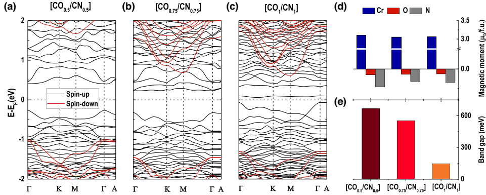
FIG. 4. Evolution of band structures with layer thickness. (a)–(c) Band structures of the \text{Cr}_2\text{O}_3/\text{CrN} SLs with CO and CN layer thickness ranging from 0.5 to 1 nm, respectively. The black and red curves represent the spin-up and spin-down states, respectively. (d) Magnetic moments for the Cr, O, and N ions and (e) the band gaps calculated for a series of [\text{CO}_t/\text{CN}_t] SLs. The band gap is defined by the difference between the eigenvalues at the bottom of conduction band and the top of valence band.
