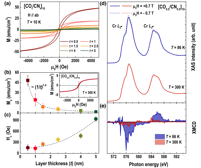
FIG. 2. Magnetometry and XMCD measurements for Cr 2 O 3 /CrN SLs. (a) In-plane M - H curves for symmetric [CO t /CN t ] 10 SLs at 10 K. (b) M_S and (c) H_C as a function of layer thickness. Inset: M - H loops for [CO 0.5 /CN 0.5 ] 10 SL at 300 K. (d) XAS at Cr L edges for [CO 0.5 /CN 0.5 ] 10 with in-plane fields of \pm 0.7 T. (e) XMCD at 86 and 300 K.
