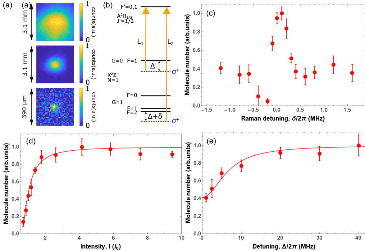
FIG. 1. 1D optical lattice loading aided by GMC. (a) YO cloud at different stages. From top to bottom are dual-frequency MOT, compressed MOT assisted by GMC, and lattice. (b) GMC configuration of YO. The cooling beams consist of two frequency components addressing G = 0, F = 1 and G = 1, F = 2 manifolds. The single-photon and two-photon detuning are denoted by \Delta and \delta , respectively. (c) Number of loaded molecules versus two-photon detuning \delta with I = 14I_0 and \Delta = 8.3\Gamma , where I_0 = 2.7 \text{ mW/cm}^2 is the estimated saturation intensity, and \Gamma = 2\pi \times 4.8 \text{ MHz} is the natural linewidth of A^2\Pi_{1/2} . (d) Number of loaded molecules versus GMC intensity I with \Delta = 8.3\Gamma and \delta = 2\pi \times 70 \text{ kHz} . (e) Number of loaded molecules versus \Delta with I = 5.5I_0 and \delta = 2\pi \times 70 \text{ kHz} . The solid lines in (d) and (e) are fits to N = N_0 - k \times \rho_{ee} , where N_0 is a constant, k is a scale factor, and \rho_{ee} is the excited state A^2\Pi_{1/2} population [as a function of I in (d) and \Delta in (e)] calculated with a three-level model (see Ref. [35]) using the corresponding experimental parameters. The error bars in the plots correspond to 1\sigma statistical uncertainty.
