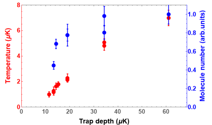
FIG. 4. Molecule cooling inside the optical lattice by ramping down the trap depth. The horizontal axis shows the final trap depth after the ramping. The red and blue dots represent the measured temperatures along the transverse direction and the numbers of the remaining molecules after trap depth ramping, respectively. The ramping may not be fully adiabatic. We observe a nearly constant or slightly increased PSD if we assume the temperature along the longitudinal direction is the same as the transverse direction.
